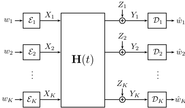
Fig. 1. K -user interference channel with fading.
