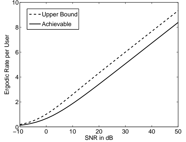
Fig. 2. Ergodic symmetric rate per user and upper bound for the K -user Gaussian interference channel with equal transmit powers: \text{SNR}_1 = \text{SNR}_2 = \dots = \text{SNR}_K .
