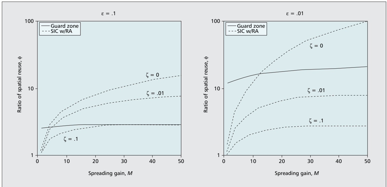
■ Figure 6. Guard zone performance vs. SIC as measured by the efficiency of spatial reuse \phi , for moderate ( \epsilon = .1 ) and severe ( \epsilon = 0.01 ) outage constraints. The baseline case of no spreading, scheduling, or SIC, is \phi = 1 .
