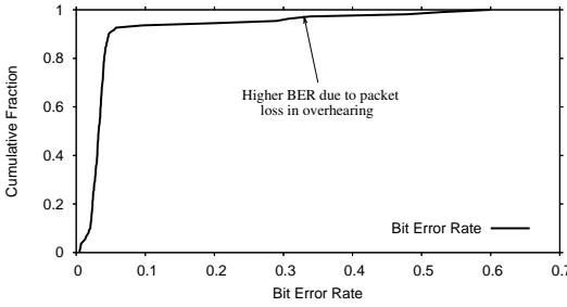
(b) CDF of BERs for “X” topology
