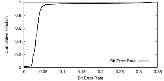
(b) CDF of BERs for Alice-Bob topology
